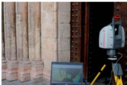
Figure 2: HDS ScanStation 2 during the data acquisition
